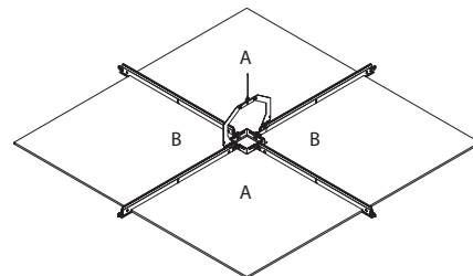
Intersection Downlighting Assembly with Calla Notched Ceiling Panels
