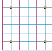
2' x 2' Ceiling layout with lights 8' apart
