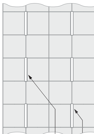
Opening for on-center linear light fixture placement
