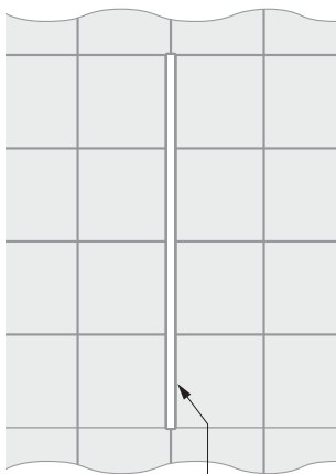
Opening for on-center linear light fixture placement
