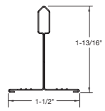
ShortSpan Tee
