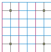
2' x 2' Ceiling layout with lights 8' apart
