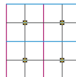
30" x 30" Ceiling layout with lights 5' apart
