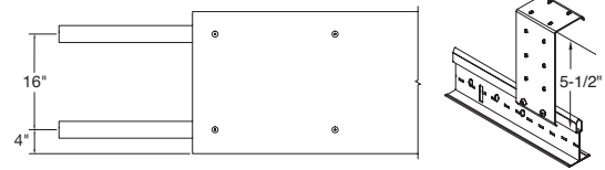
Wall, deck, or I-beam installation using FrameAll™ Drywall Grid and uptight clips
