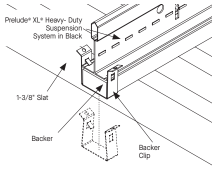
Ceiling Backer Assembly
