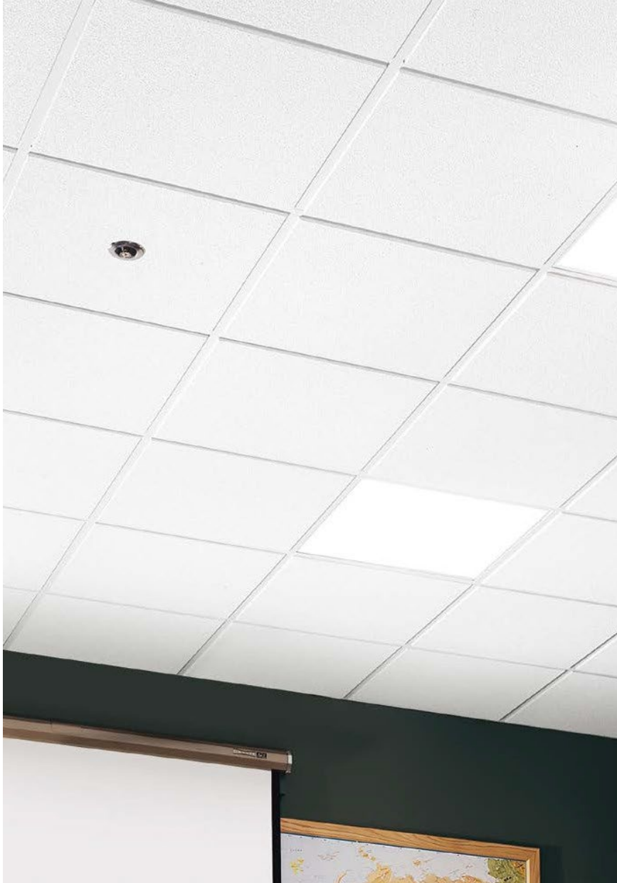
Georgian™ Beveled Tegular panels with Prelude® XL® 15/16" suspension system
