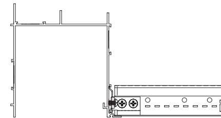
AXTBC standard clip, suspension system flush
