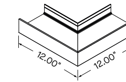
Knife Edge Ceiling-to-Ceiling Outside Corner
