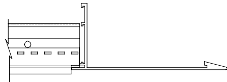
Tegular Panel
