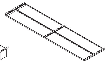
6372AC1M1 Panel 12" Wide 1" Deep – 2 Planks
