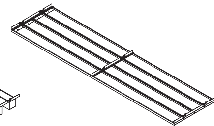
6374A61M1 Panel 6" Wide 1" Deep – 4 Planks
