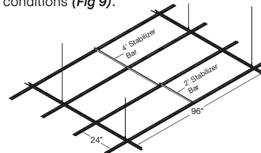
24" x 96" Panel Installation
