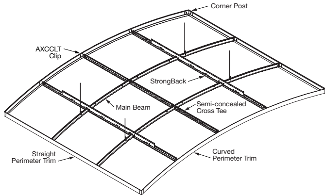
Assembly Drawing (one main beam long)
