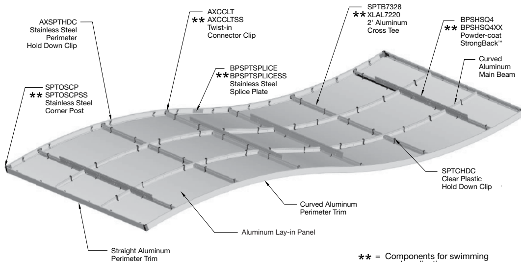
Assembly Drawing for Above a Pool (144" x 72" module, 630 H/V main beam, 24" x 24" lay-in panel)
