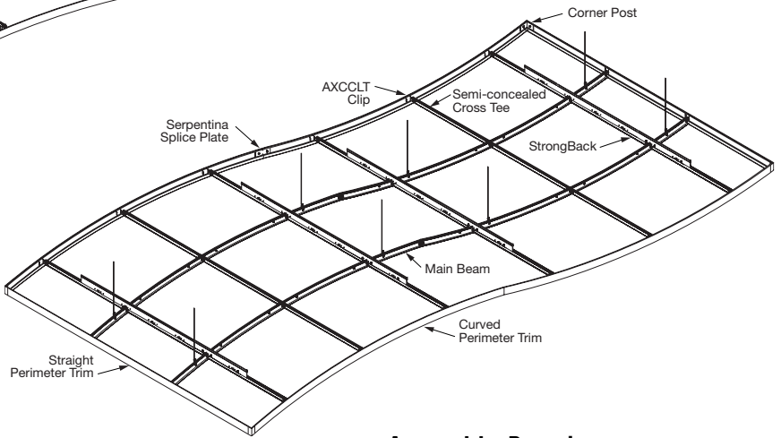
Assembly Drawing (main beams connected end to end)
