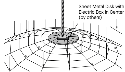
Electrical Box
