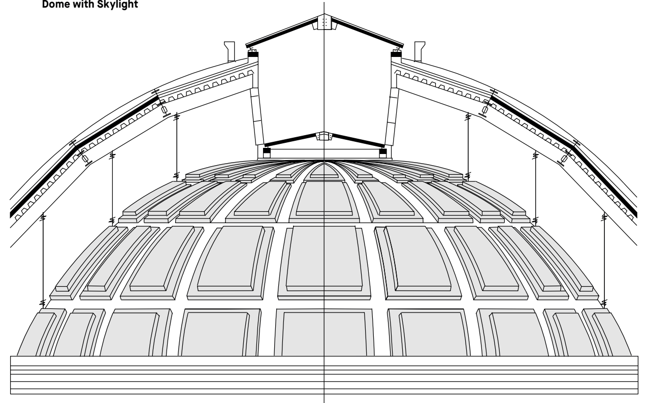
Dome with Skylight
