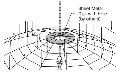
Electrical Chain
