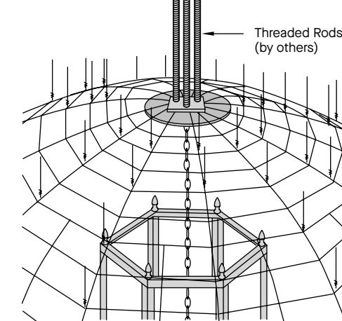
Light Fixture
