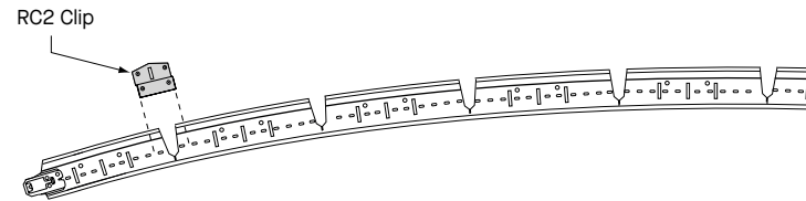
Radius and drywall thickness will determine on-center spacing of cuts. Refer to "Establishing An Arc" on page 9 for creating a curved template.
