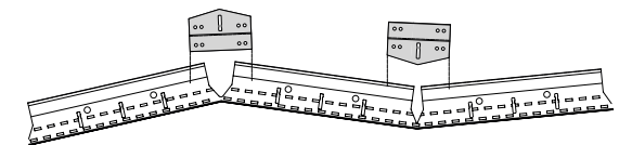
* RC2 Clip placement Vaults - Cross tee placement in routs between cuts. Valleys - Cross tee lock into rout on RC2 clip (tight radius installations may require bending up of the flange at ends of cross tees).
