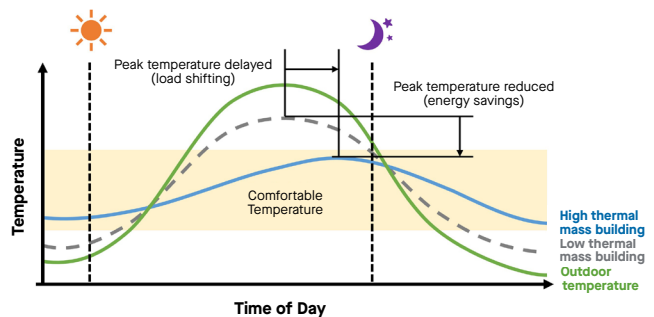
Illustration of temperature variation in thermally massive and light buildings in a climate with warm days and cool nights
