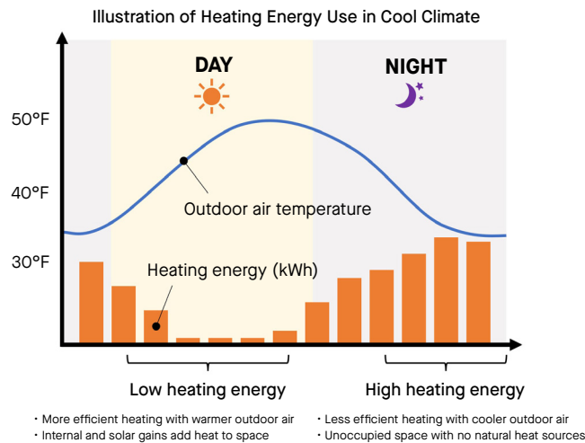
Figure 1. Illustration of energy saving mechanism of thermal mass in a cool climate in a building with high daytime gains.
