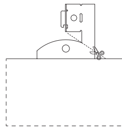
Blade panel with hardware attached to Axiom molding
