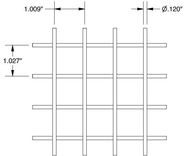
DETAIL A WIRE SPACING DETAIL SCALE 1 : 2
