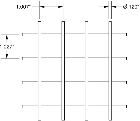
DETAIL A WIRE SPACING DETAIL SCALE 1 : 2
