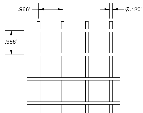
DETAIL A WIRE SPACING DETAIL SCALE 1 : 2
