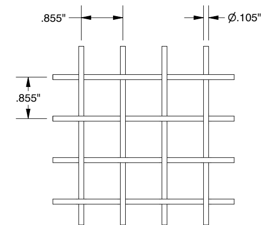
DETAIL A MESH SPACING DETAIL SCALE 1 : 2
