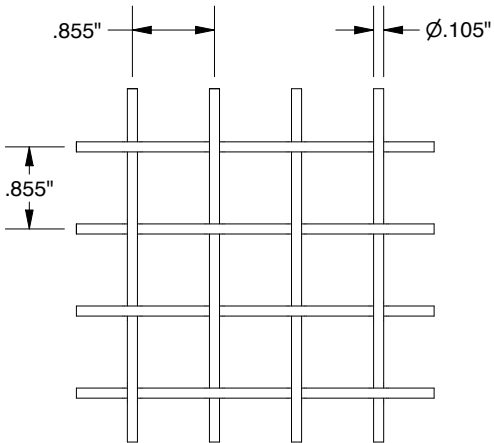
DETAIL A MESH SPACING DETAIL SCALE 1 : 2
