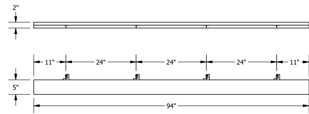
BP8250F03RH06-??? Painted Rectangular Vertical Panel 94in Length 5in Depth
