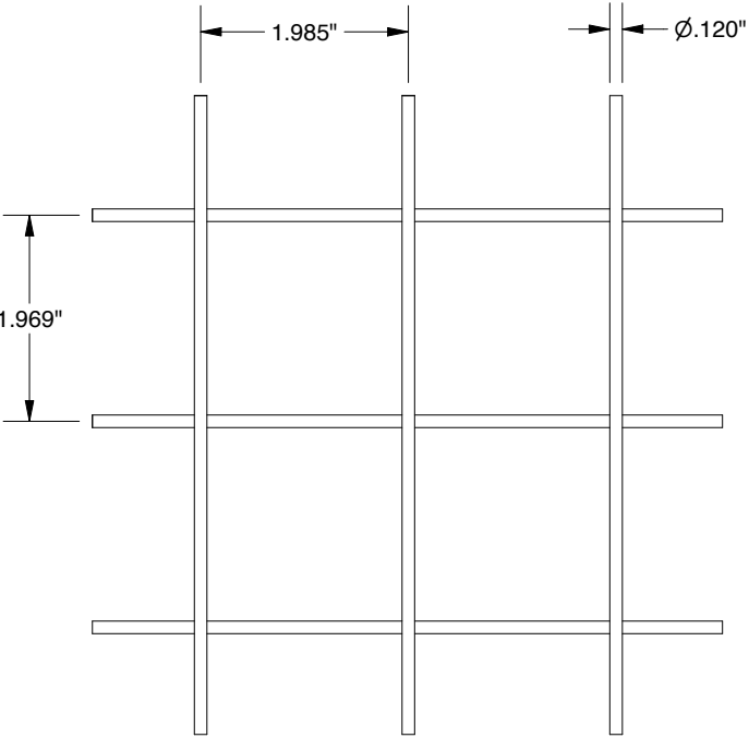
DETAIL A WIRE SPACING DETAIL SCALE 1 : 2
